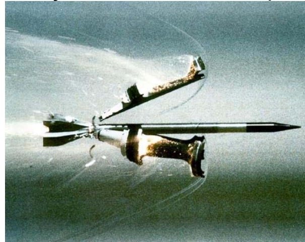
Projatil 120 mm anti-tanque
